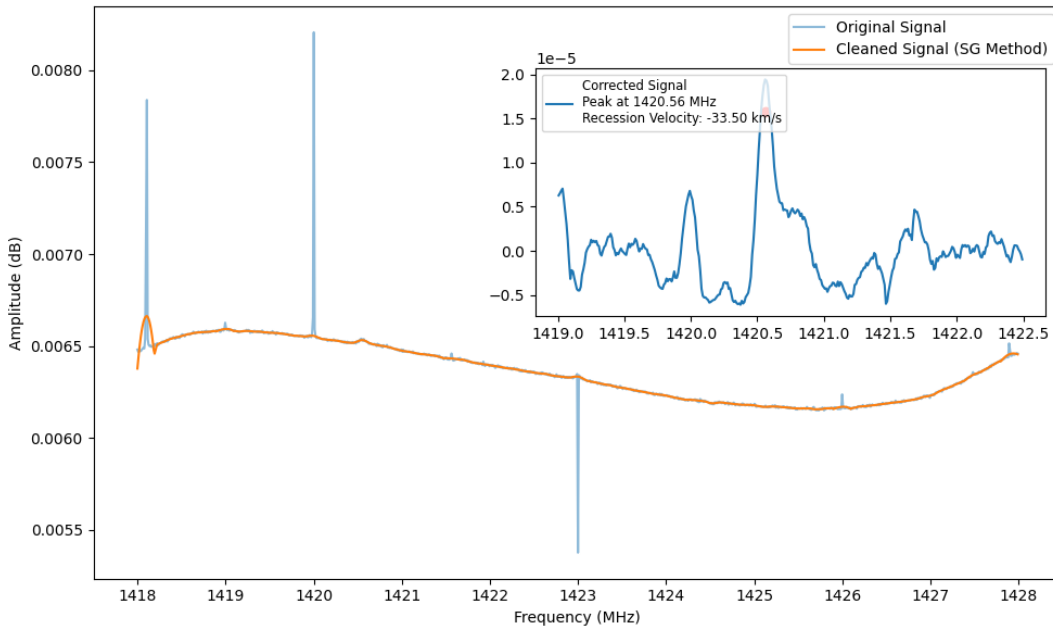
Figure 2: Graph of all data files from the August 12th 2024 session. The ROI Inset shows peak at 1420.56 MHz with a recession velocity of -33.50 km/s.
