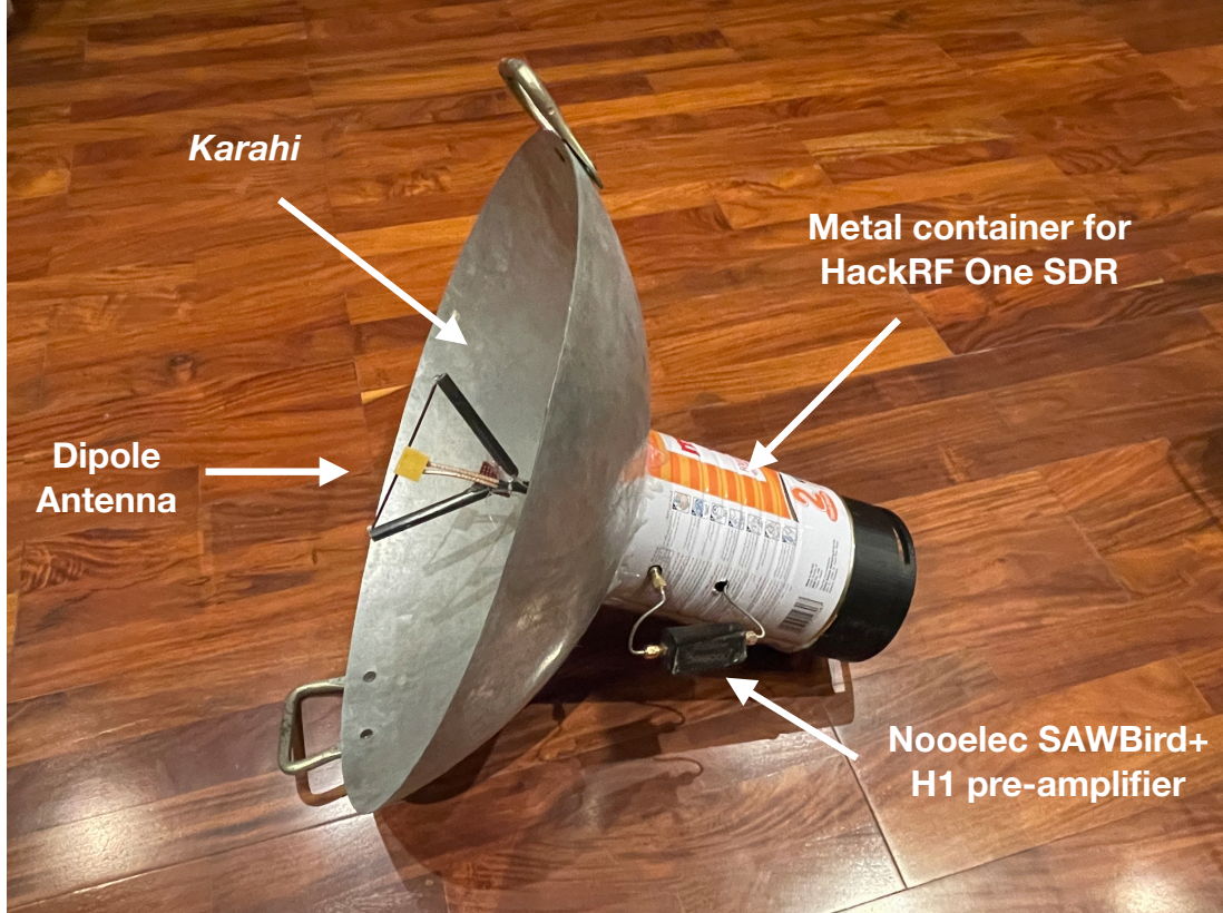
Figure 1: The setup of the galactic dish system (dubbed the karahi ).
